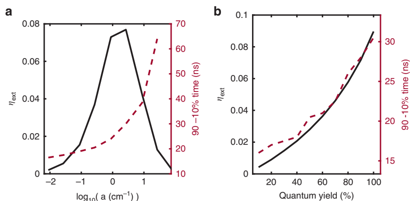
Fig. 5 Effects of luminescent solar concentrator parameters on impulse response. a (Black solid line) simulated external optical efficiency, \eta_{\text{ext}} , as a function of the logarithm of the absorption coefficient of the devices for fixed device parameters. (Red dashed line) simulated fall time of the impulse response of devices as a function of the logarithm of the absorption coefficient. b (Black solid line) simulated external optical efficiency, \eta_{\text{ext}} , as a function of quantum yield for a Lumogen Red 305-doped device with fixed concentration and dimensions. (Red dashed line) simulated fall time of the impulse response as a function of quantum yield
